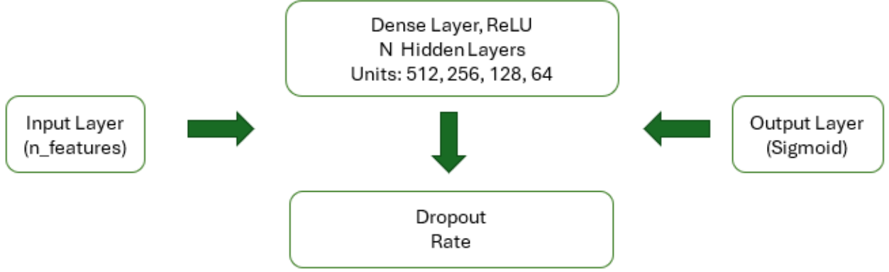
Figure 5: DNN Architecture
